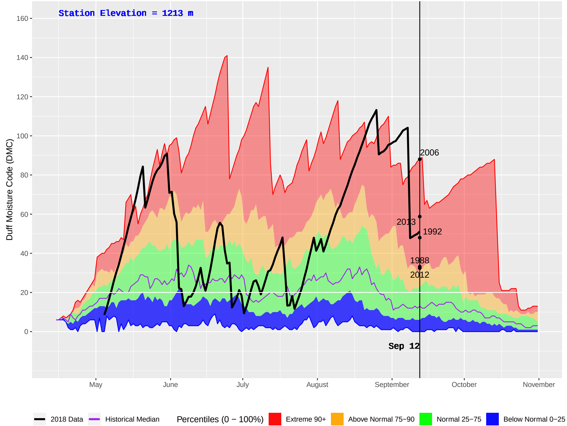
INGENIKA POINT (145) : Historical (1971–2016) and Current (2018) Daily Duff Moisture Code (DMC)
