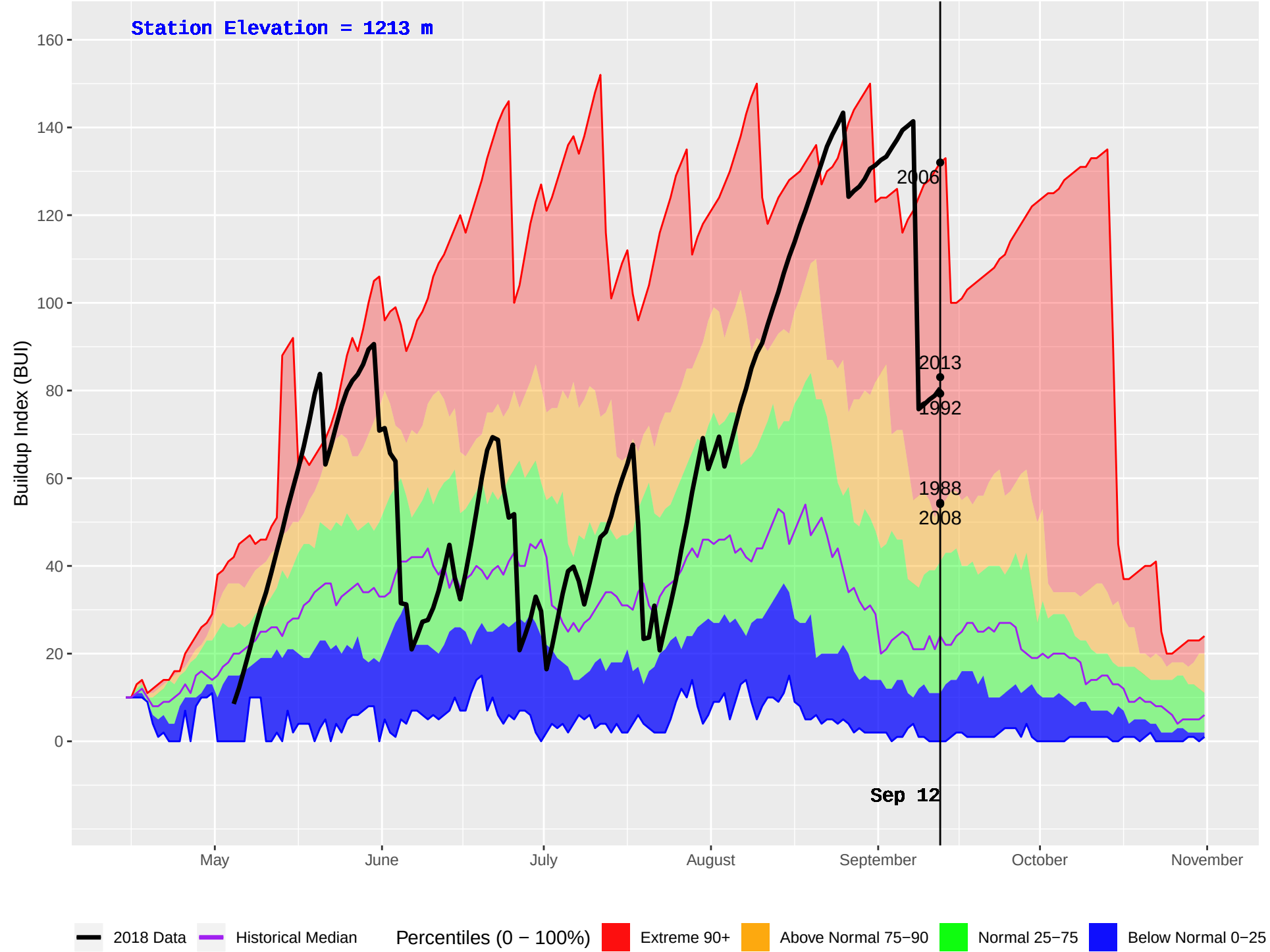
INGENIKA POINT (145) : Historical (1971–2016) and Current (2018) Daily Buildup Index (BUI)
