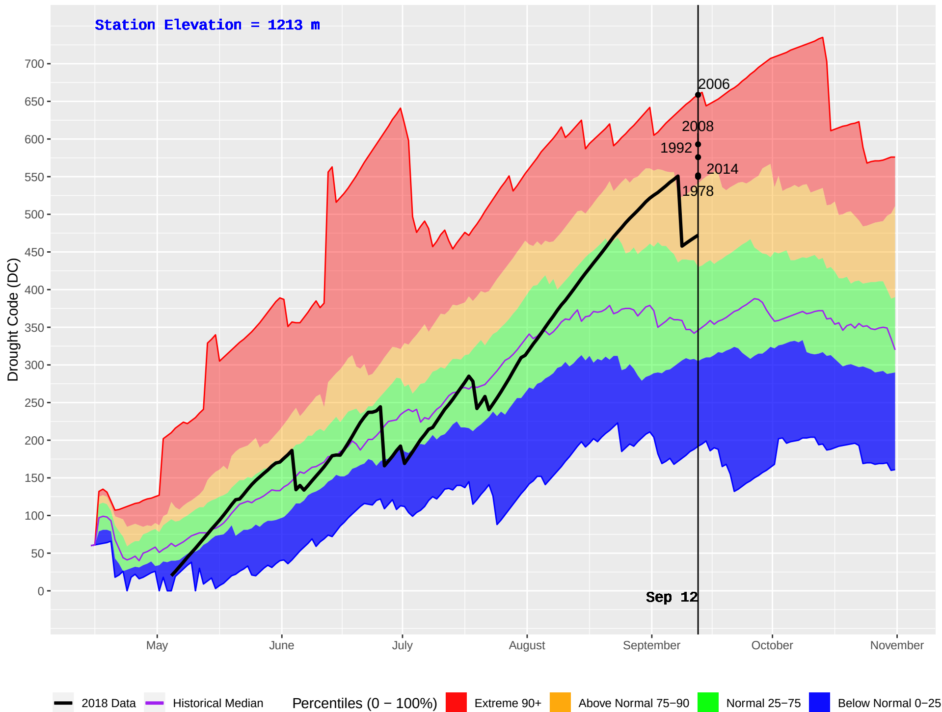
INGENIKA POINT (145) : Historical (1971–2016) and Current (2018) Daily Drought Code (DC)
