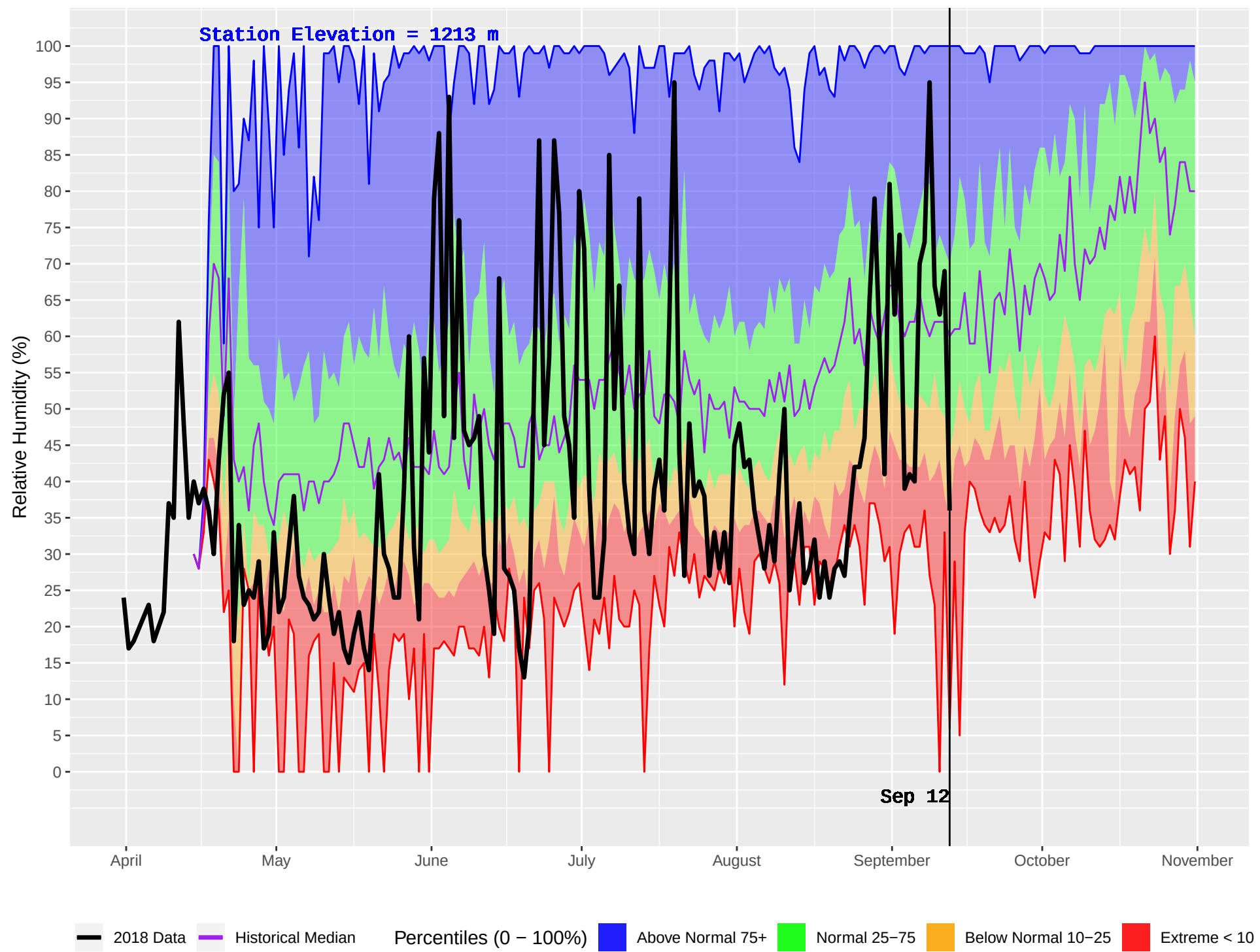
INGENIKA POINT (145) : Historical (1971–2016) and Current (2018) Daily Relative Humidity
