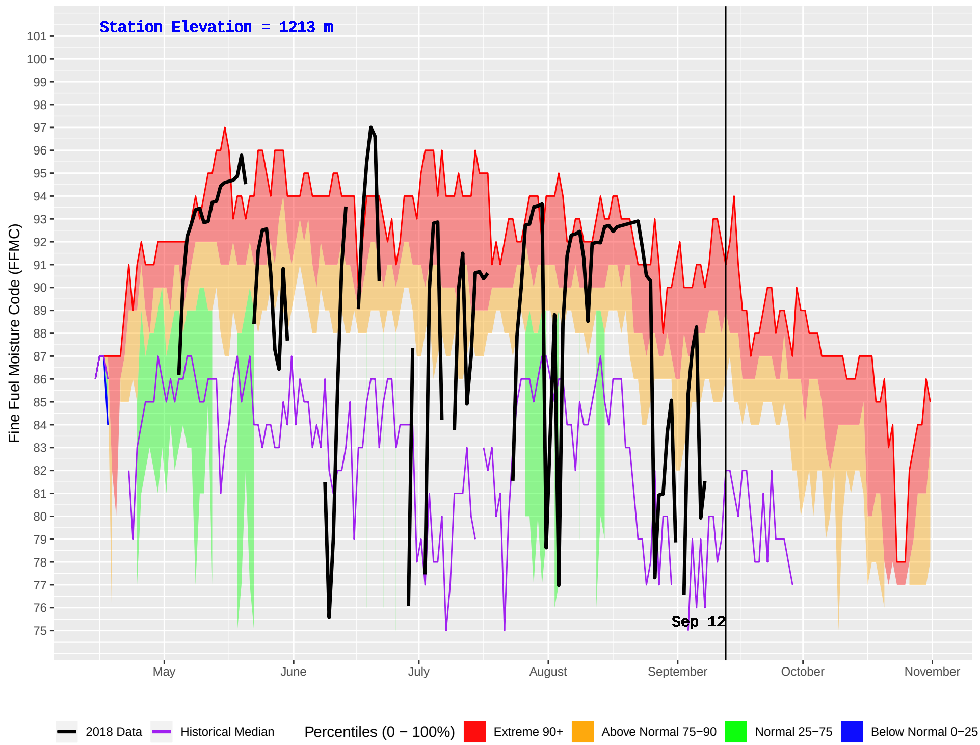
INGENIKA POINT (145) : Historical (1971–2016) and Current (2018) Daily Fine Fuel Moisture Code (FFMC)
